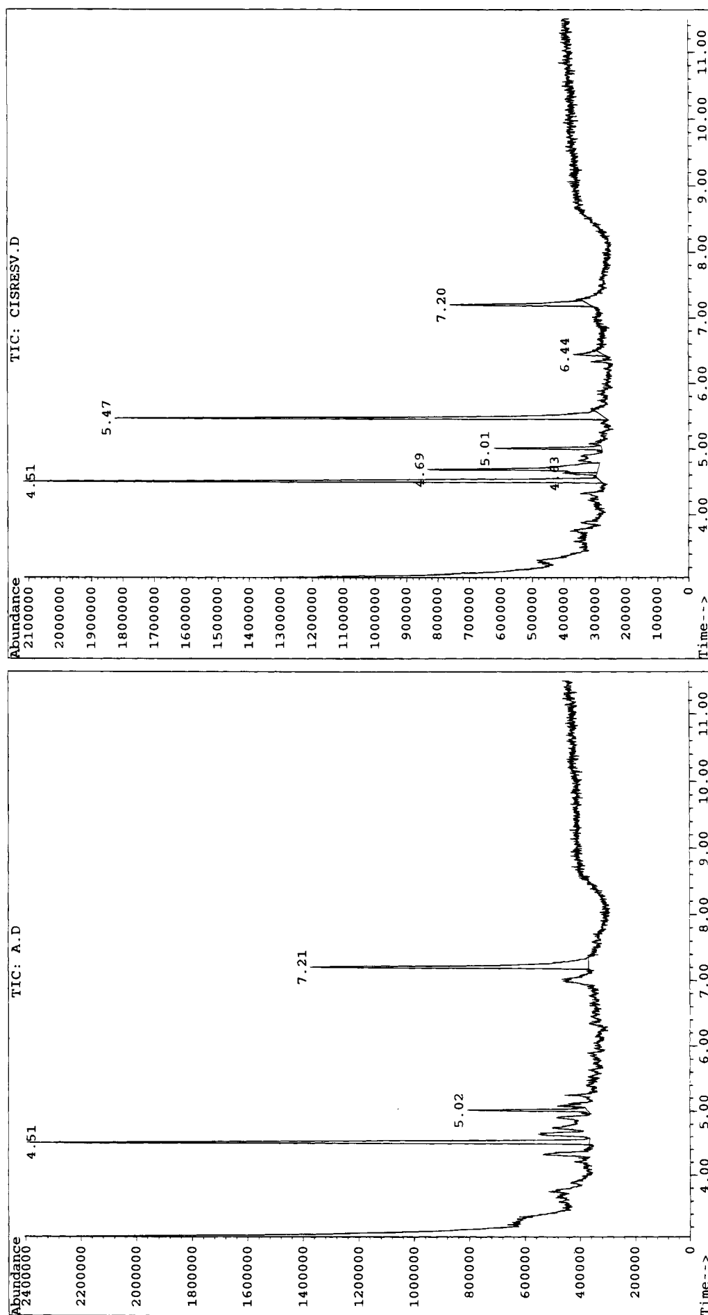
Figure 2. (A, Left) Total ion spectrum of a red wine eluate with no detectable cis - or trans -resveratrol (Californian Red Burgundy, nonvintage). (B, Right) Total ion spectrum of eluate of same wine to which cis -resveratrol (prepared by irradiation of a solution of
